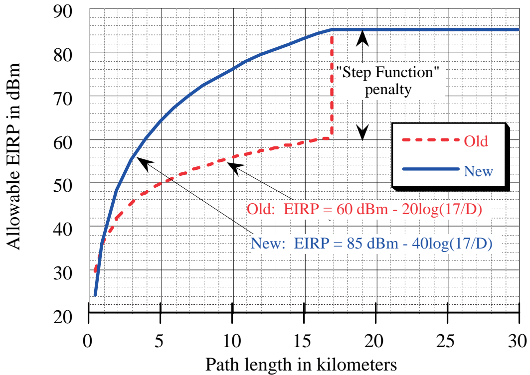
Figure 1. Graph showing the old vs. new minimum path length EIRP formula for the 7 GHz TV BAS band. Similar EIRP restrictions apply to fixed links in the 2, 2.5 and 13 GHz TV BAS bands.
